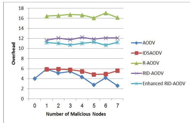
Figure. 11: Overhead Ratio vs. number of malicious nodes for different protocols
