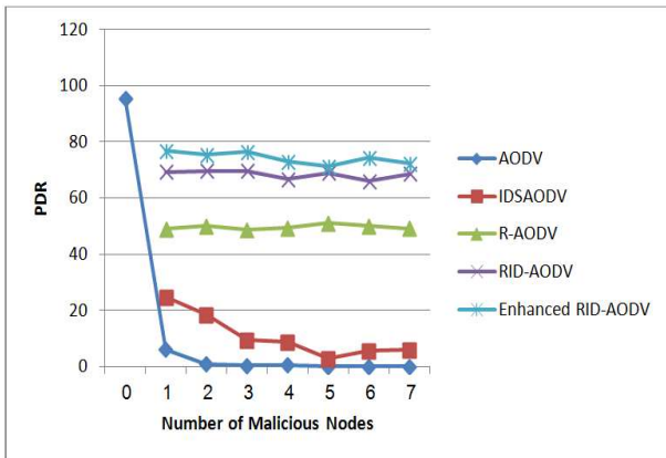
Figure. 9: PDR vs. number of malicious nodes for different protocols
