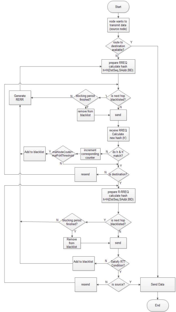
Figure. 7: Flowchart of the Enhanced RID-AODV protocol
