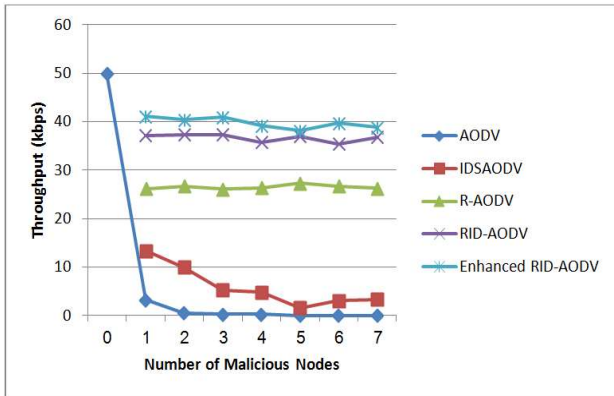
Figure. 8: Throughput vs. number of malicious nodes for different protocols
