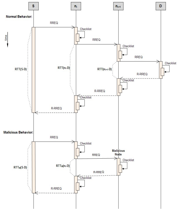
Figure. 3: Sequence Diagram for the Enhanced RID-AODV
