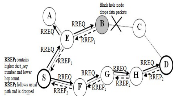
Figure. 1: Black Hole Attack Illustration
