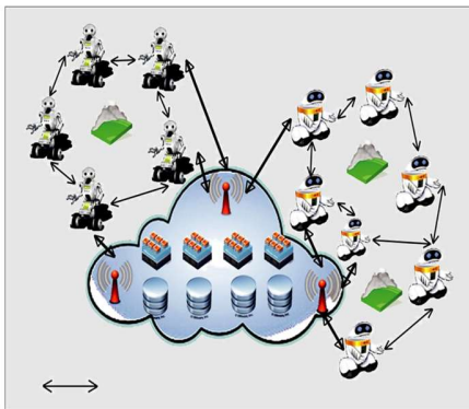
Figure 2. Cloud Robotics: robots are interconnected via M2M/M2C communications, sharing their resources and accessing to remote cloud resources. Machine-to-cloud (M2C), Machine-to-machine (M2M)
