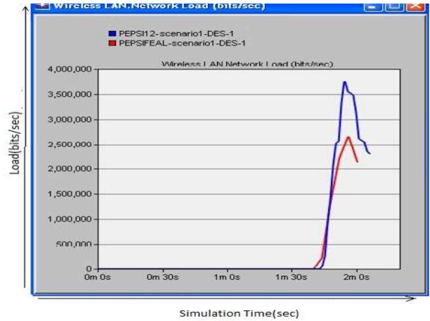
Figure 4: Proposed Load
