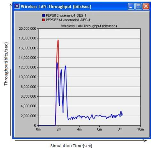
Figure 5: Proposed Throughput
